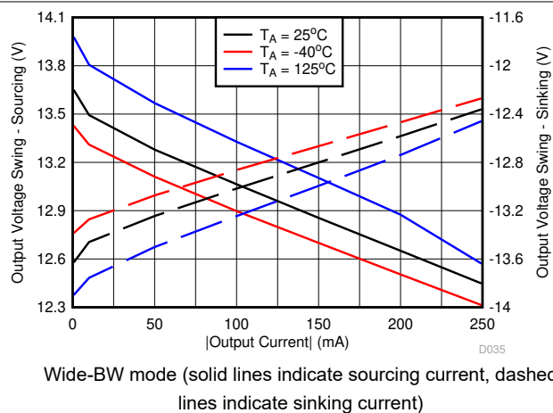
图 7-17. Output Voltage Swing vs Output Current
