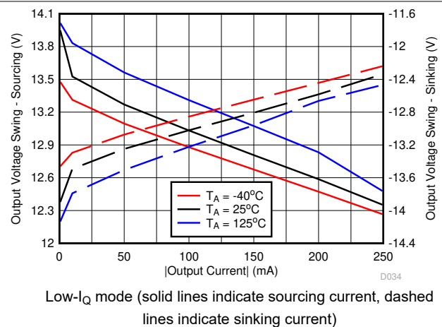
图 7-18. Output Voltage Swing vs Output Current
