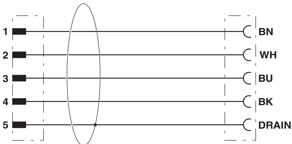
Circuit diagram
